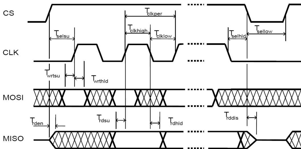
Figure 7. SPI Interface Timing Diagram
