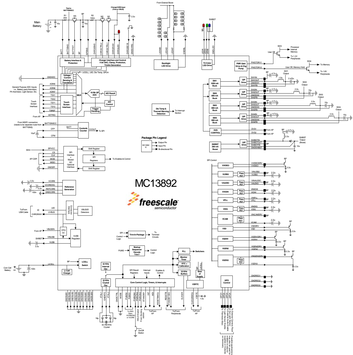
Figure 35. 13892 Typical Application
